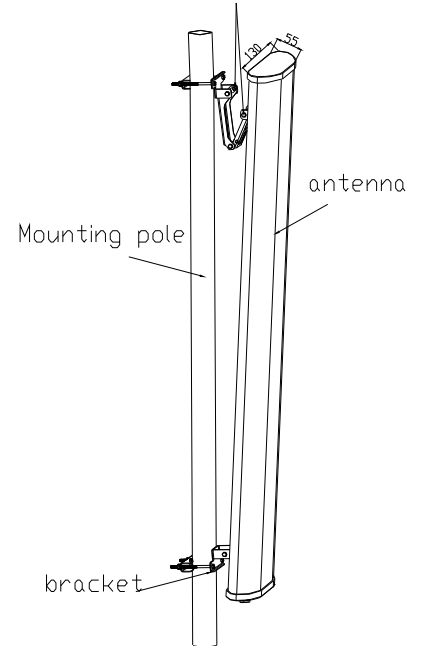
Adjusting bracket
